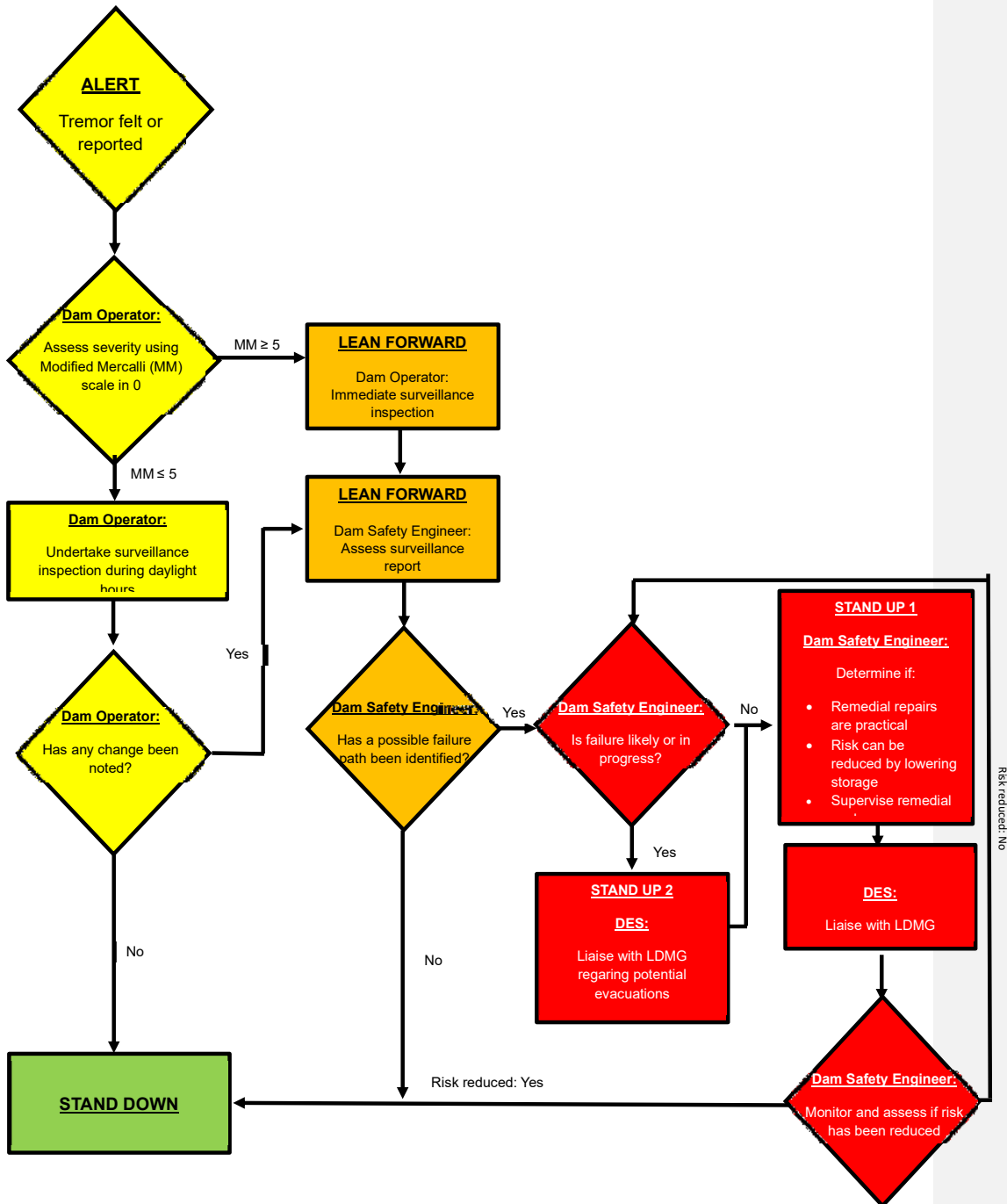
FIGURE 5-2 EARTHQUAKE FLOWCHART
