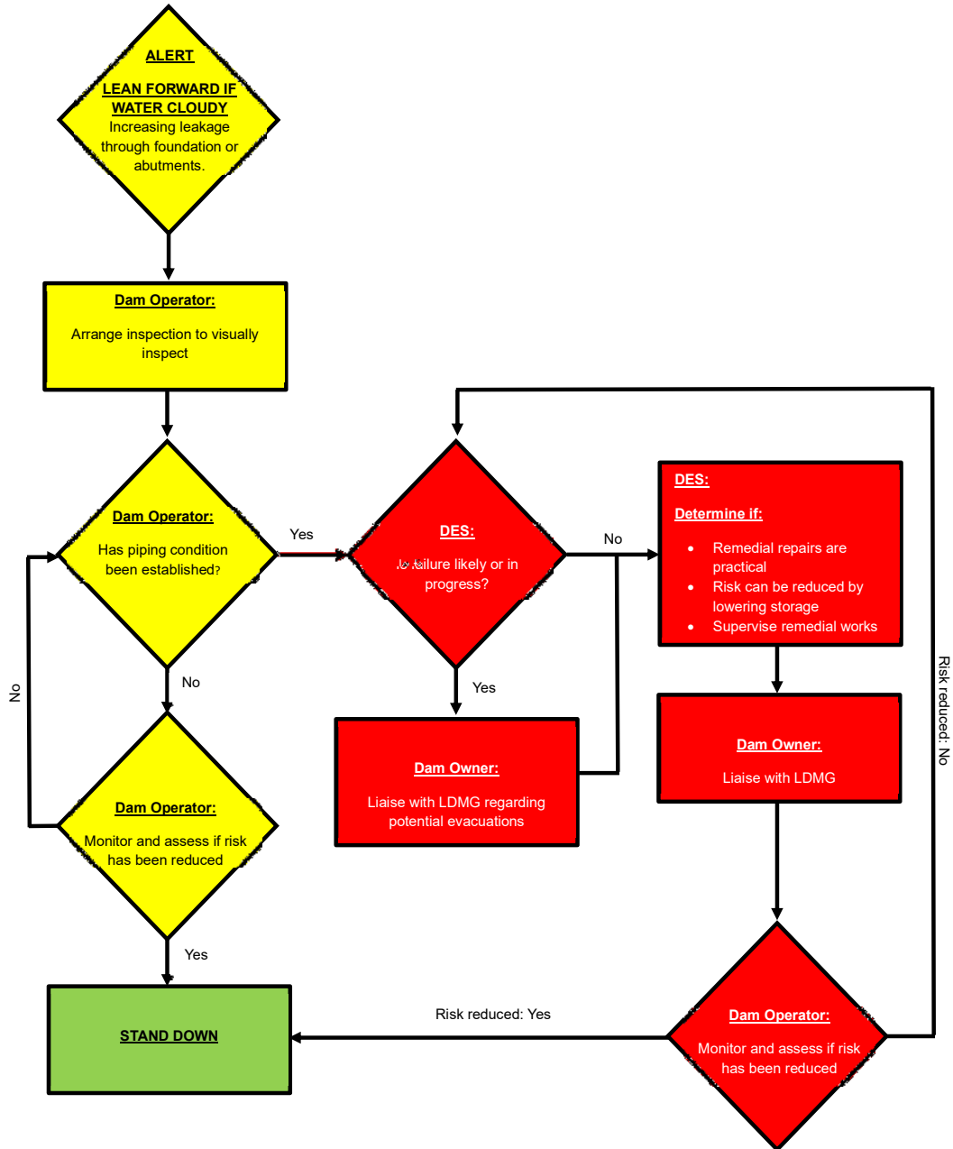
FIGURE 5-3 PIPING: EMBANKMENT, FOUNDATION OR ABUTMENTS FLOWCHART
