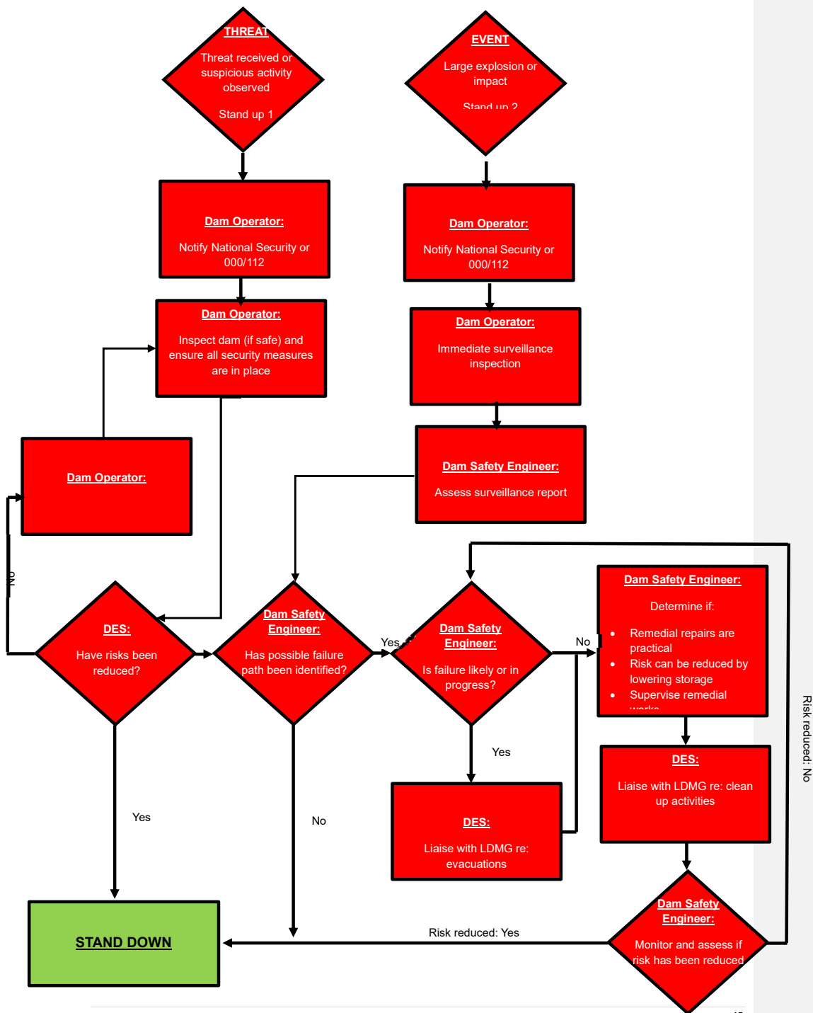
FIGURE 5-4 TERRORIST THREAT/ACTIVITY OR HIGH ENERGY IMPACT FLOWCHART
