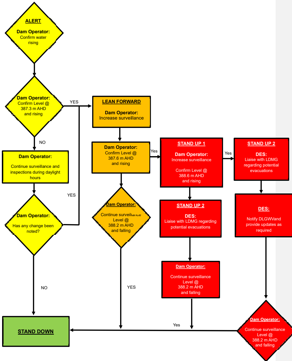
FIGURE 5-1 SIGNIFICANT FLOW THROUGH SPILLWAY FLOWCHART
